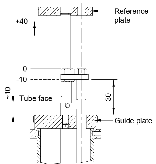
Downward borehole
