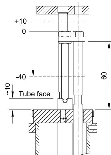
Upward borehole
