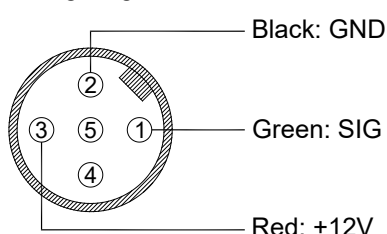
5-pin male connector Wiring diagram
