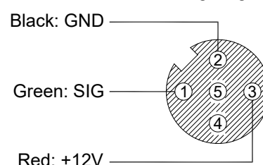
5-pin female connector Wiring diagram
