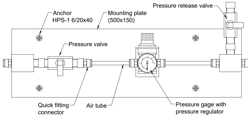
Figure 4-3 Pressure gage and valve assembly
