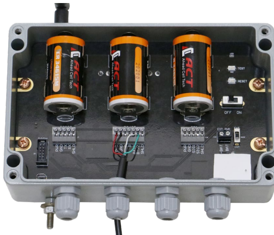
Figure 9-3 Connection of digital sensor with Modbus (RS-485) output to digital node
