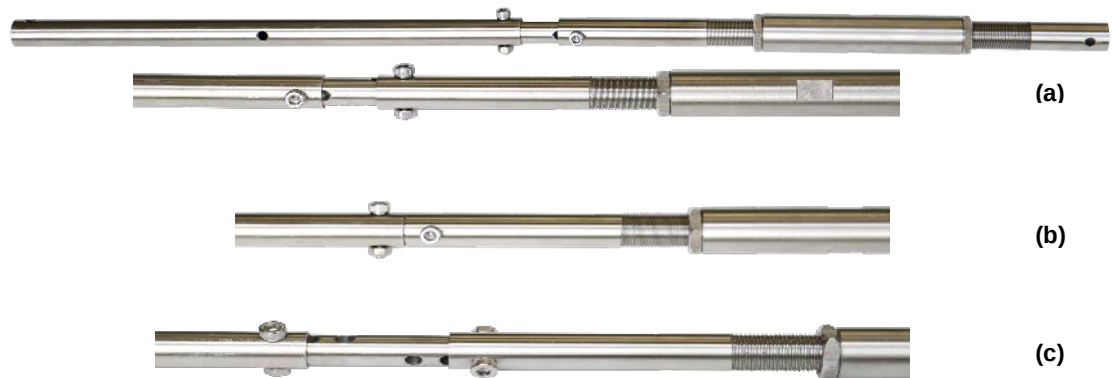
Figure 4-6 Gage coupler tubing with coarse adjustments of \pm 12.5 and \pm 25 mm through extension pin with six holes (left) and spacer tube and fine adjustments of \pm 25 mm with chuck nut with right and left hand threads (right).
