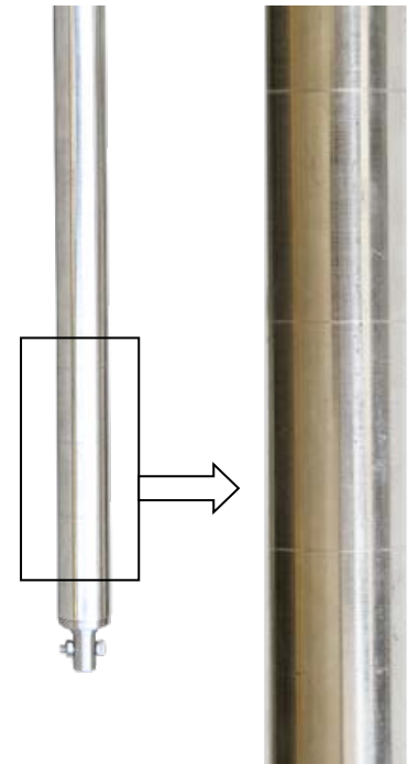
Figure 6-4 Sensor marking 100 mm for settle- ment measurement
