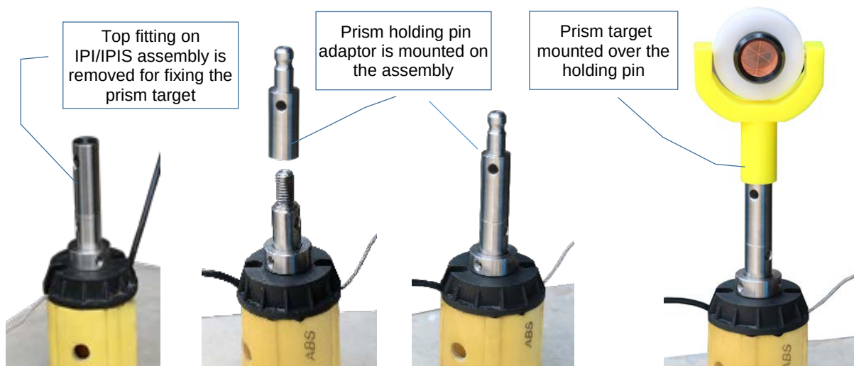
Figure 4-3 Prism target mounting accessories suitable for taking X-Y coordinates for IPIS
