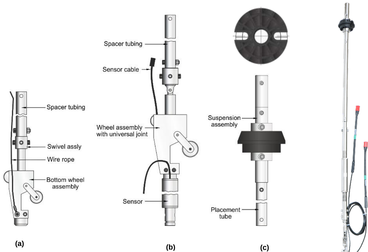
Figure 4-7 Sensor assembly
