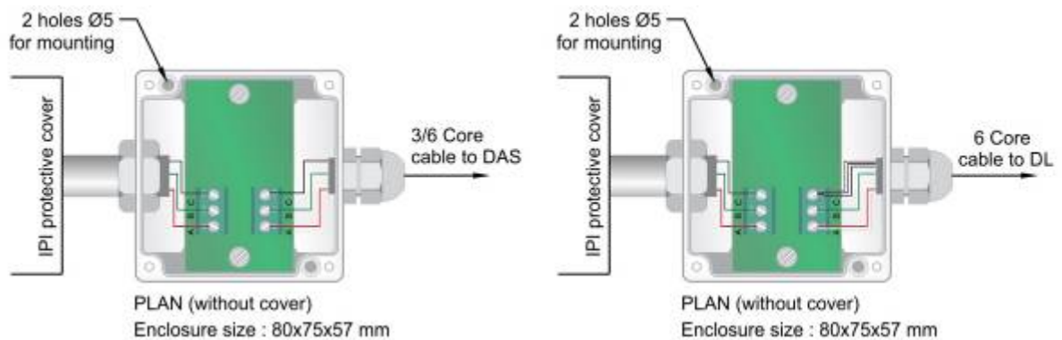
Figure 6-1 Junction box
