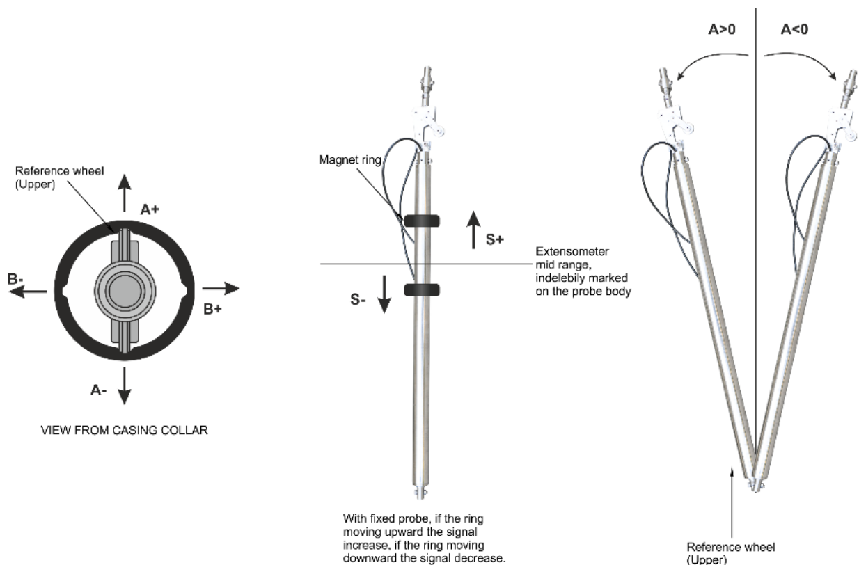
Figure 6-3 Displacement and Settlement Direction
