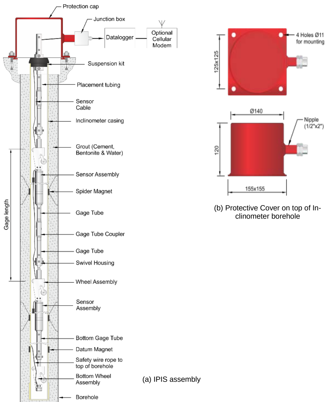
Figure 3-1: In-place 3D Inclinator cum Settlement assembly and Protective cover
