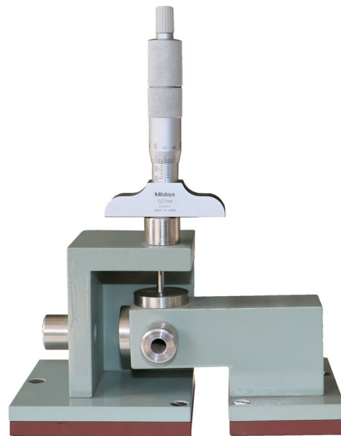
Figure 7 Taking readings using a depth gage in Z-axis
