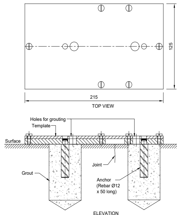
Figure 4 Details of pits for installing mounting plates
